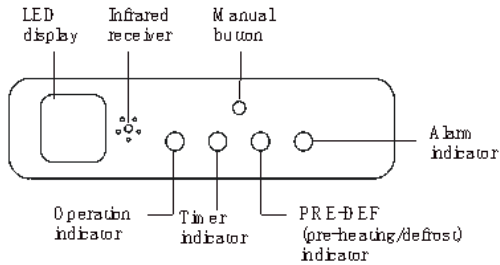
Display panel
